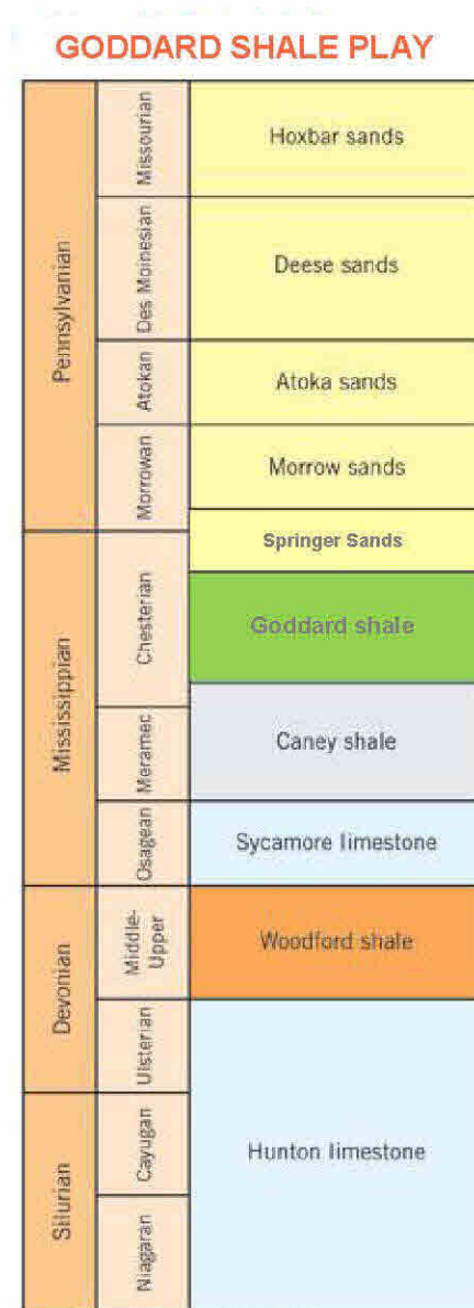
Figure 1-1 Stratigraphic Column of the South Central Oklahoma Oil Province (modified from Continental Resources, 2014).
